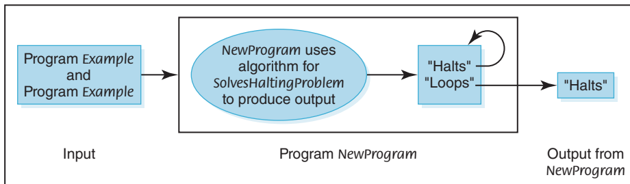
FIGURE 18.8 Construction of NewProgram
