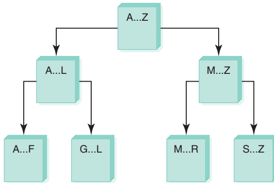
FIGURE 7.15 Ordering a list using the Quicksort algorithm
