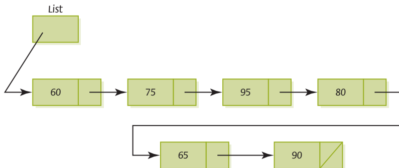
FIGURE 8.2 An unsorted linked list
