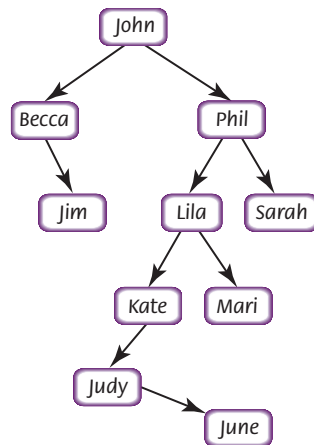
FIGURE 8.9 A binary search tree built from strings
