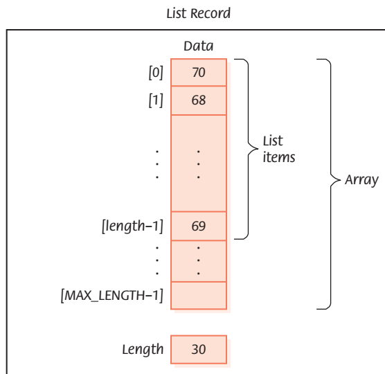
FIGURE 8.1 An unsorted list of integers
