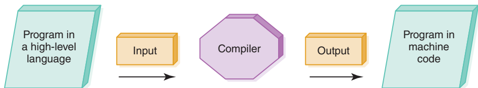
FIGURE 9.2 Compilation process
