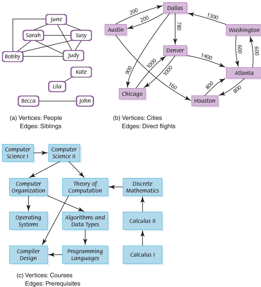
FIGURE 8.10 Examples of graphs
