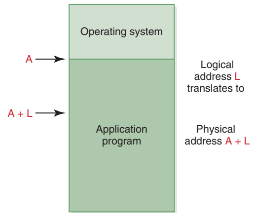
FIGURE 10.6 Binding a logical address to a physical address
