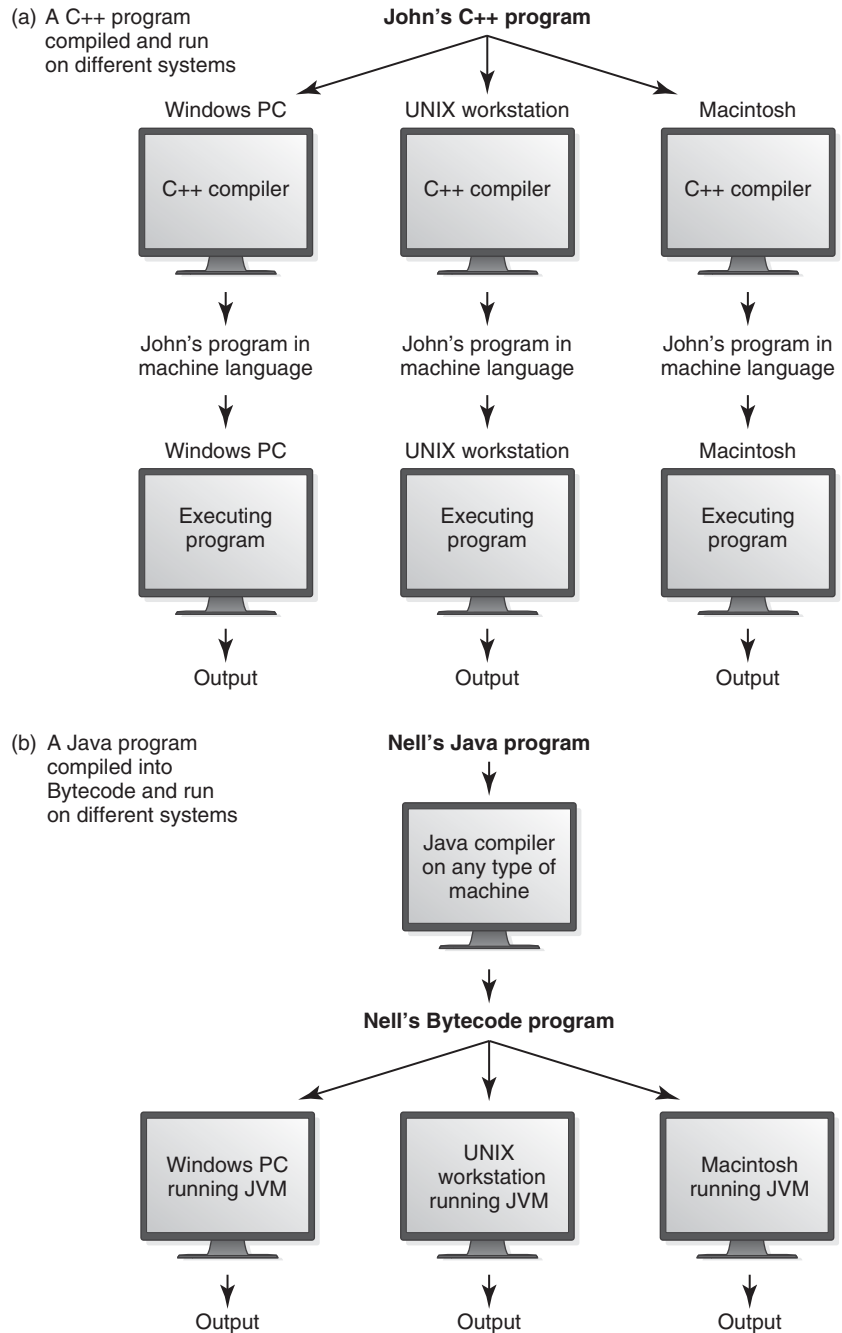
FIGURE 9.3 Portability improvement because of Bytecode interpretation
