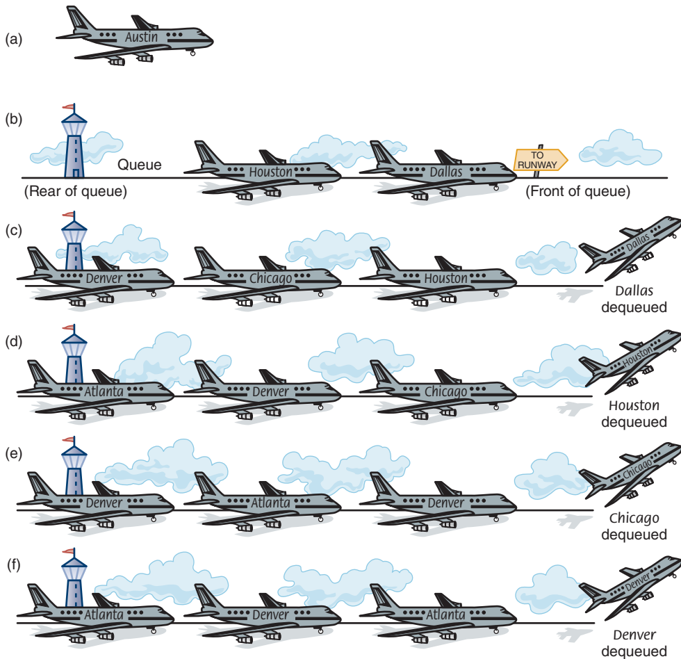
FIGURE 8.13 Using a queue to store the routes
