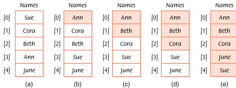
FIGURE 7.11 Examples of selection sort (sorted elements are shaded)
