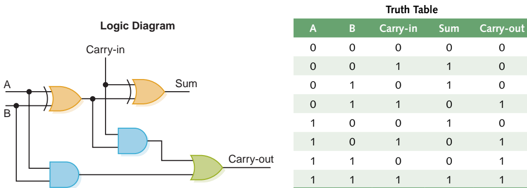
FIGURE 4.10 A full adder
