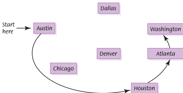
FIGURE 8.12 The depth-first search
