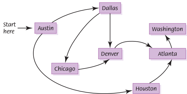
FIGURE 8.14 The breadth-first search
