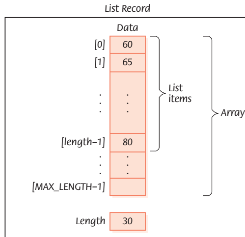
FIGURE 8.3 A sorted list of integers
