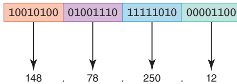
FIGURE 15.10 An IP address stored in four bytes
