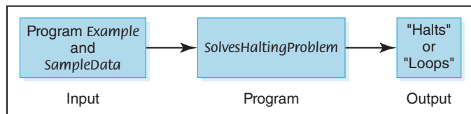
FIGURE 18.6 Proposed program for solving the halting problem
