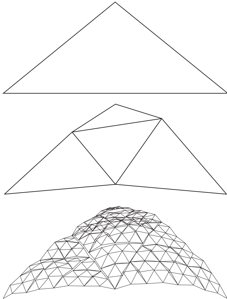
FIGURE 14.6 Midpoint sub division for creating fractal terrains
