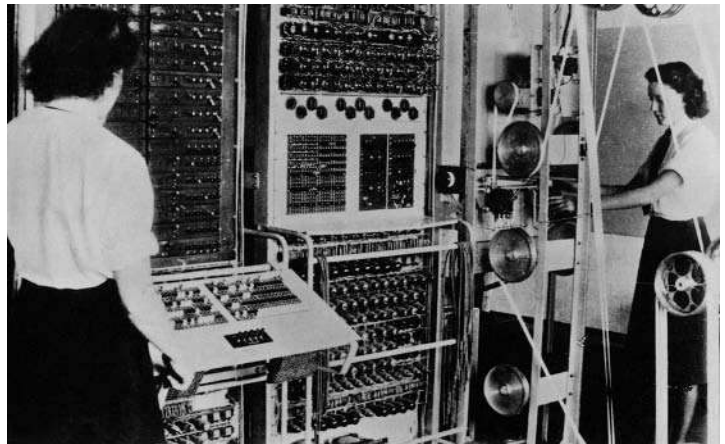
FIGURE 1.4 The Colossus, the first all-programmable digital computer
