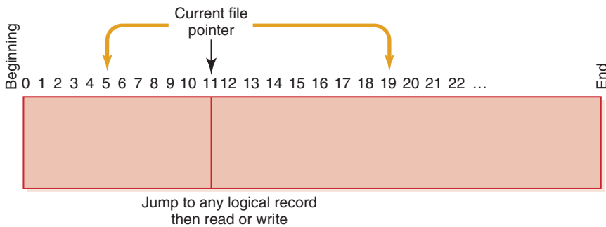
FIGURE 11.3 Direct file access
