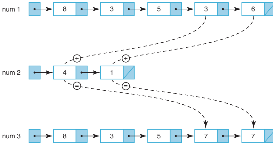
FIGURE 18.1 Representing very large numbers
