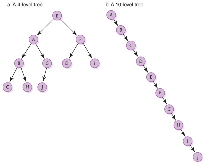
FIGURE 8.8 Two variations of a binary search tree
