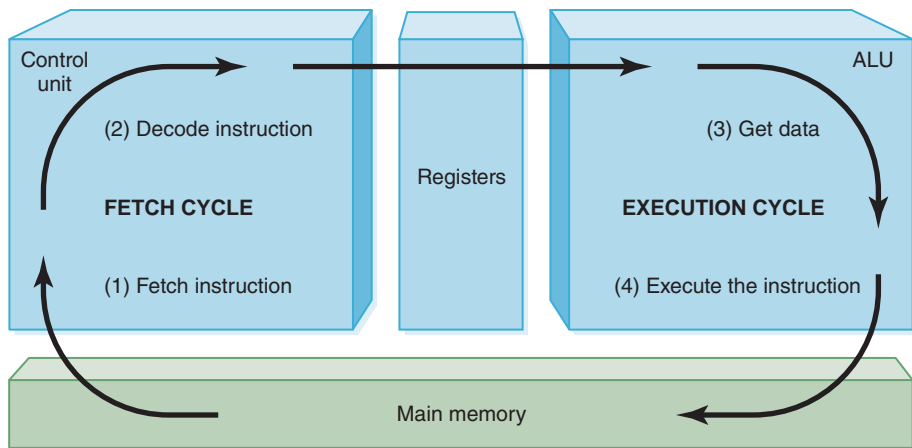
FIGURE 5.3 The fetch–execute cycle
