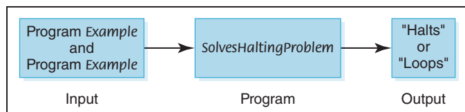
FIGURE 18.7 Proposed program for solving the halting problem
