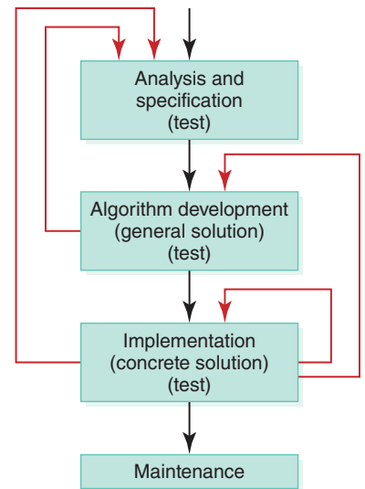
FIGURE 7.3 The interactions among the four problem-solving phases
