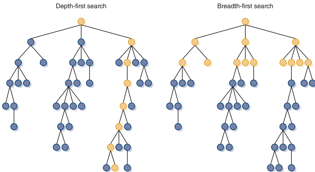
FIGURE 13.5 Depth-first and breadth-first searches
