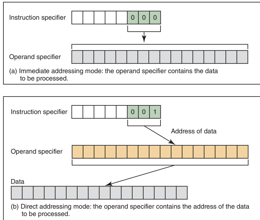
FIGURE 6.3 The difference between immediate addressing mode and direct addressing mode
