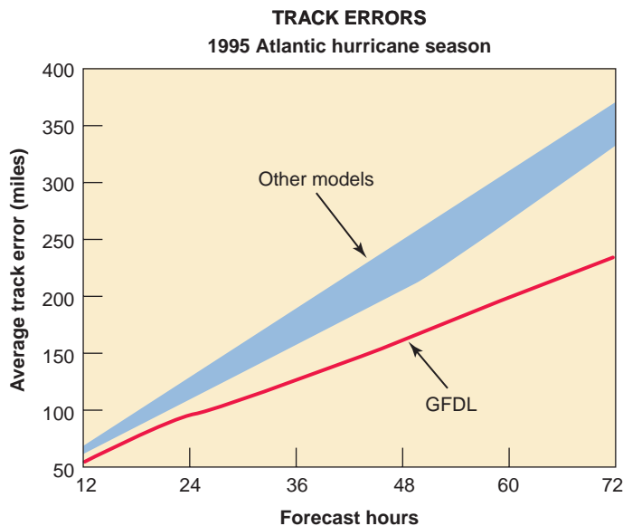
FIGURE 14.2 Improvements in hurricane models
