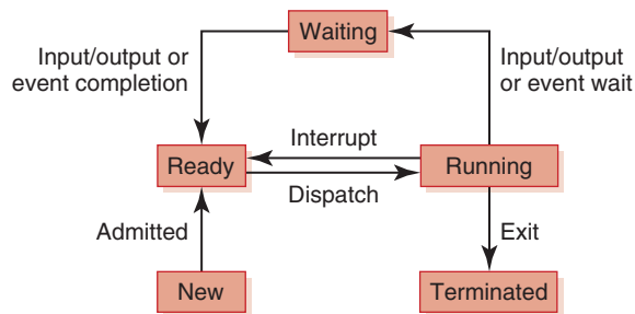
FIGURE 10.9 The process life cycle
