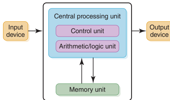
FIGURE 5.1 The von Neumann architecture
