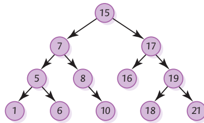
FIGURE 8.7 A binary search tree
