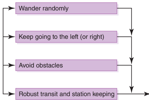
FIGURE 13.10 The new control paradigm
