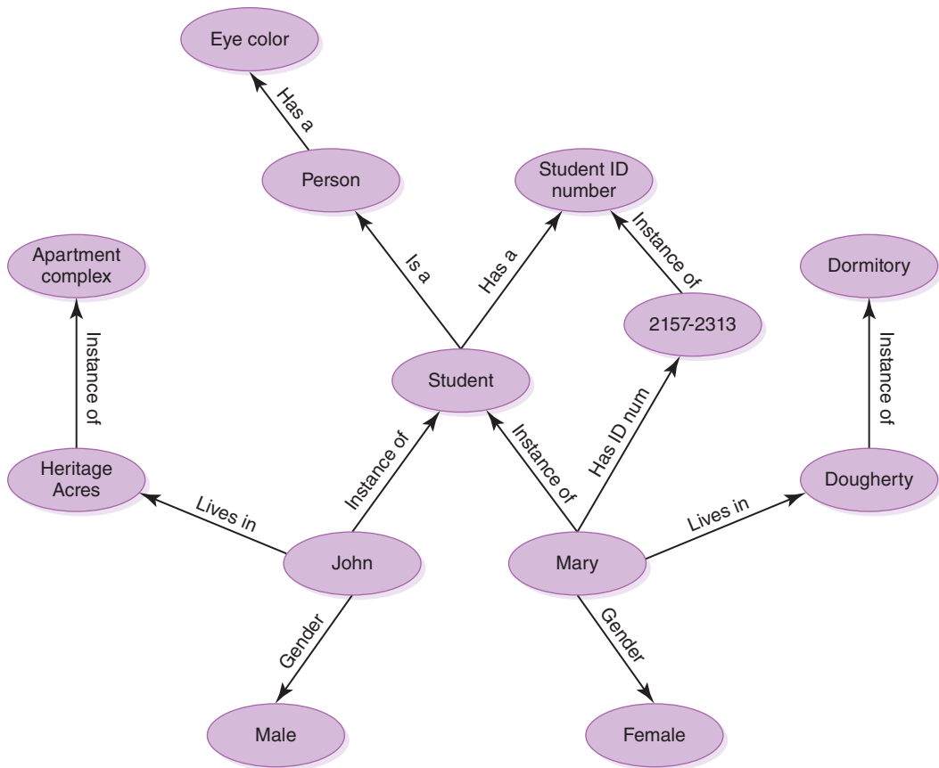
FIGURE 13.3 A semantic network
