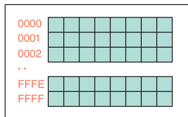
FIGURE 6.1 Pep/9's architecture
